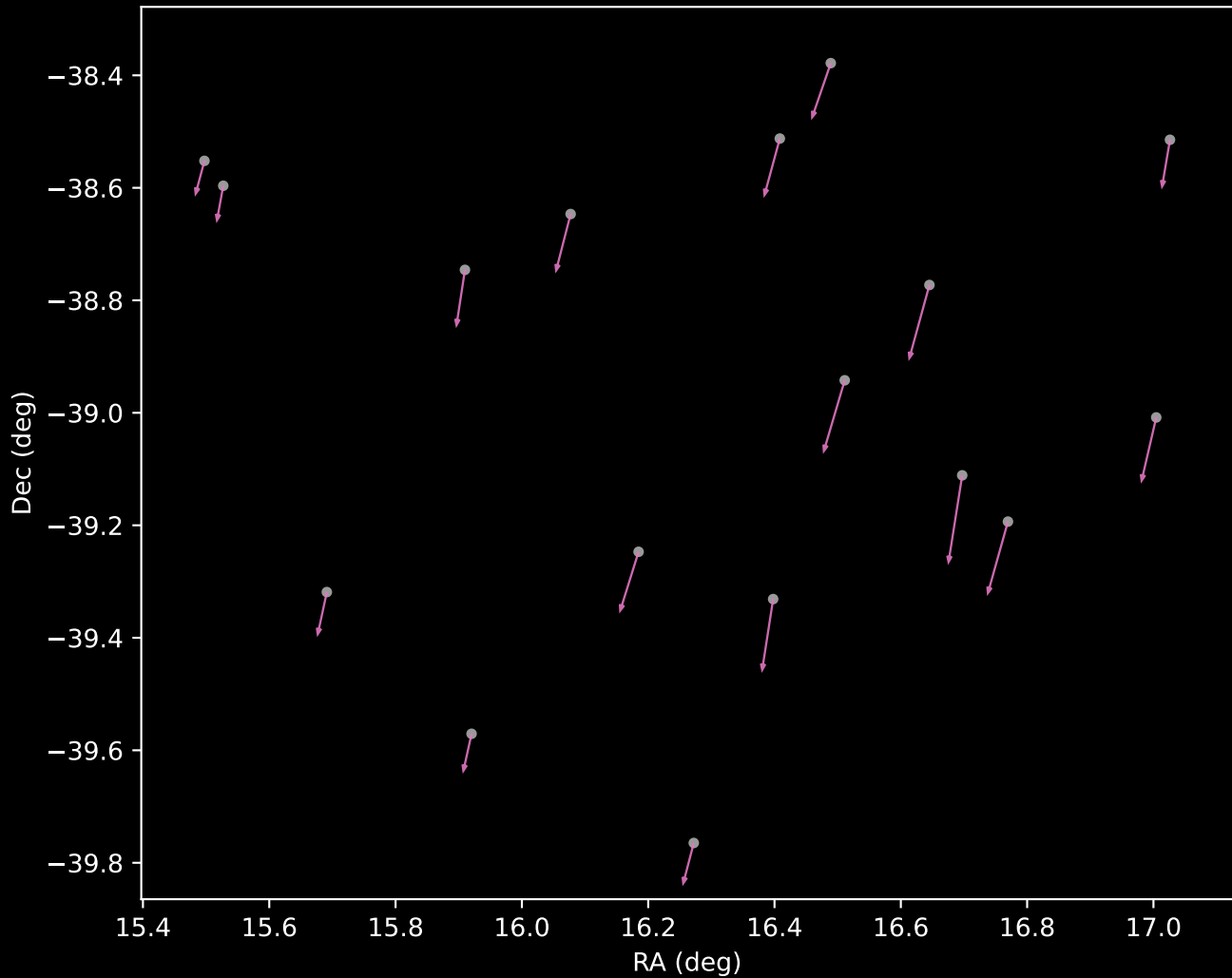
APOGEE DR17 Cluster 12 Proper Motion Vectors (n=17)
