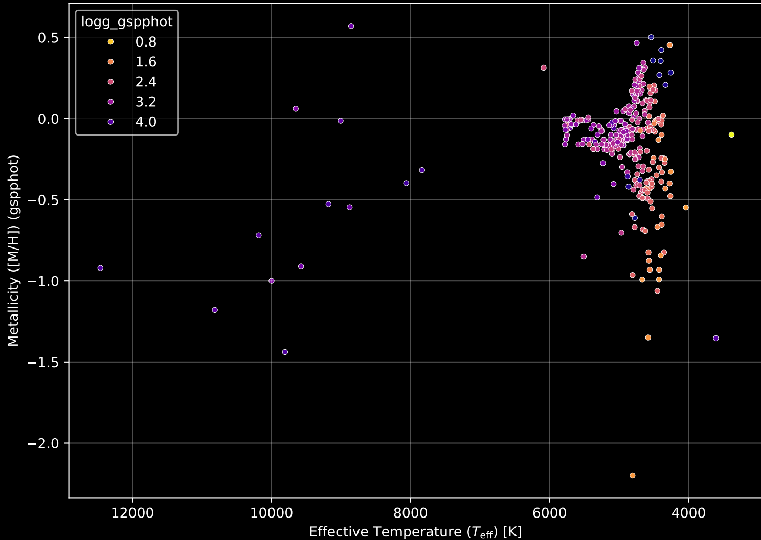
APOGEE DR17 Field: [355-12] Stellar Population Parameters (n= 328)
