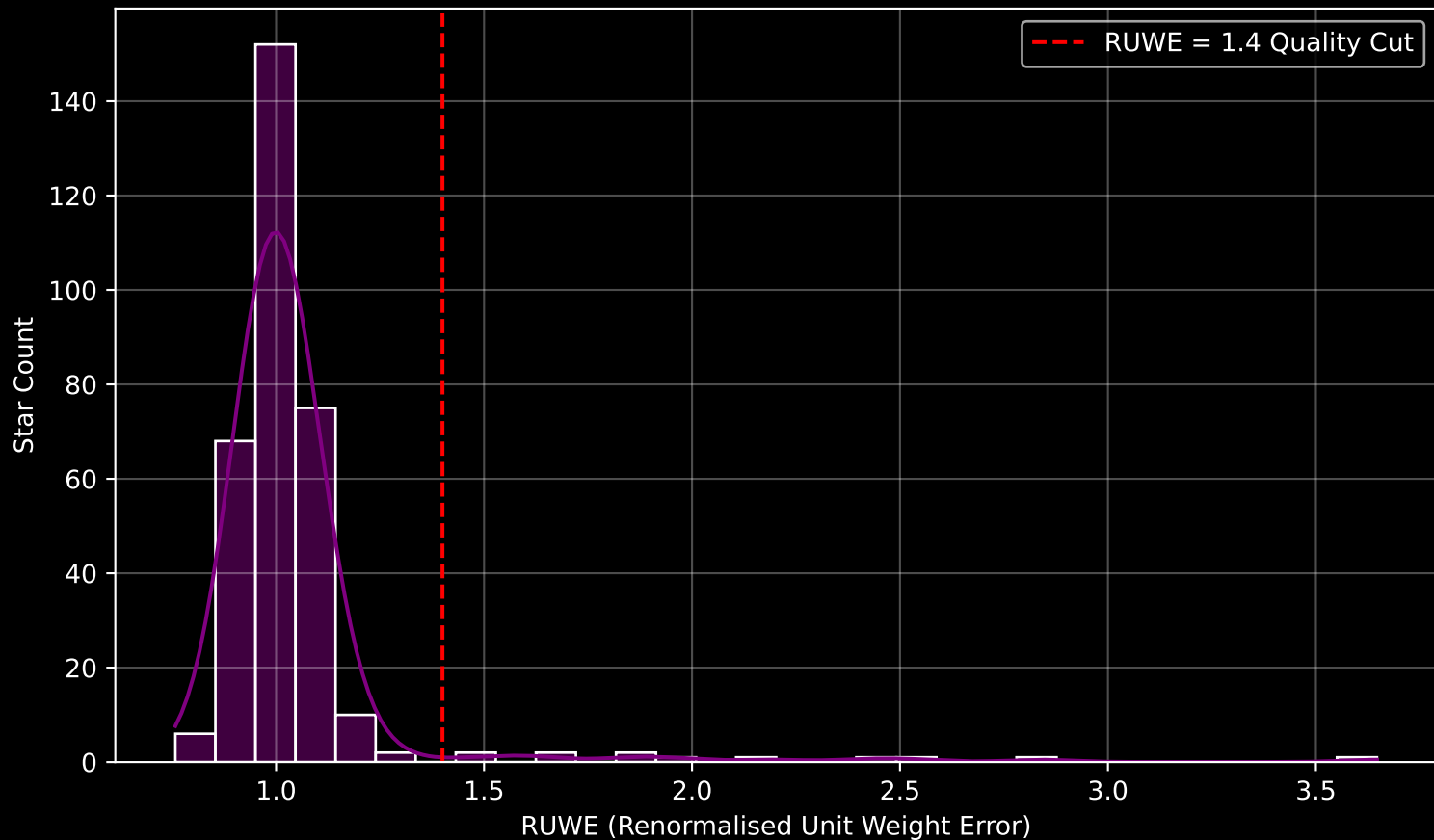
GAPOGEE DR17 Field [355-12] RUWE Distribution (n= 325)
