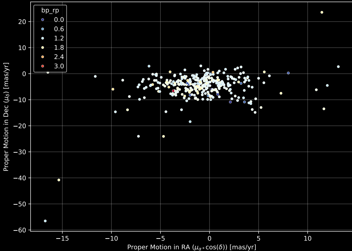
APOGEE DR17 Field: [355-12] Proper Motion Diagram (n= 328)
