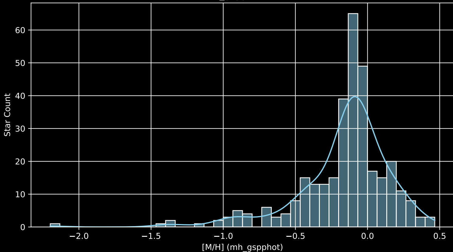
APOGEE DR17 Field: [355-12 [M/H] (mh_gspphot) (n= 326)
