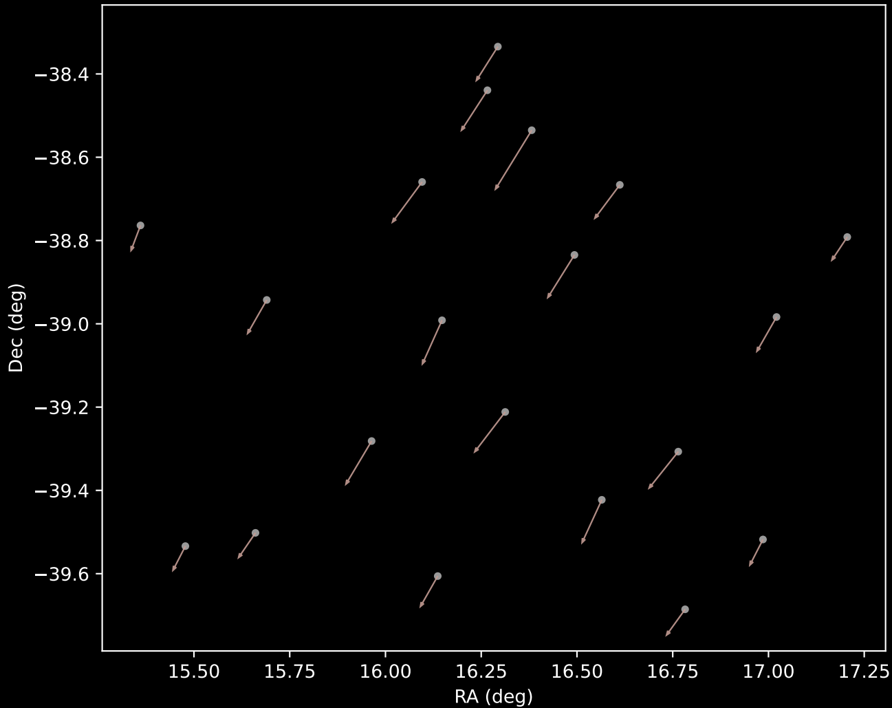
APOGEE DR17 Cluster 11 Proper Motion Vectors (n=20)
