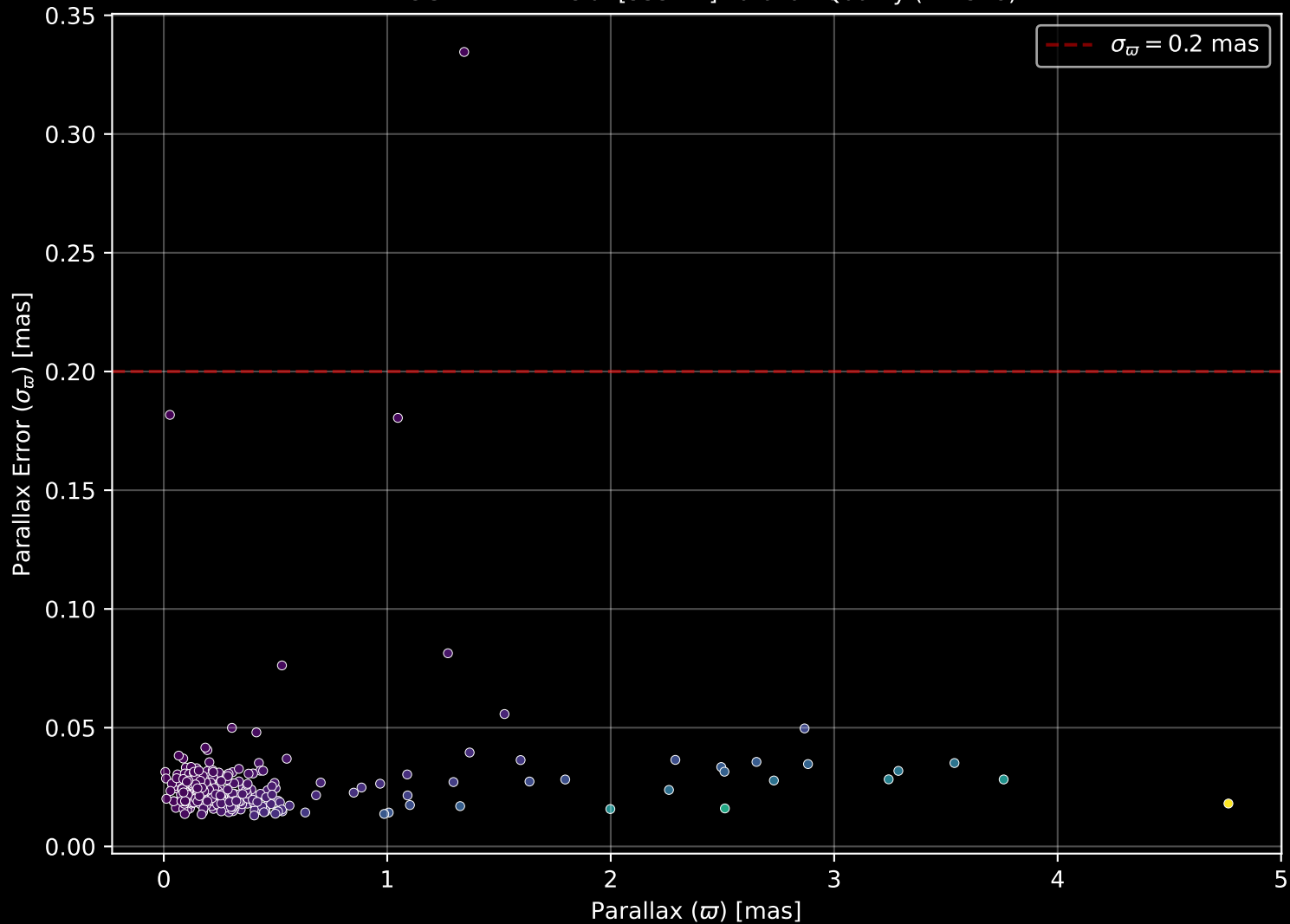
APOGEE DR17 Field: [355-12] Parallax Quality (n= 328)
