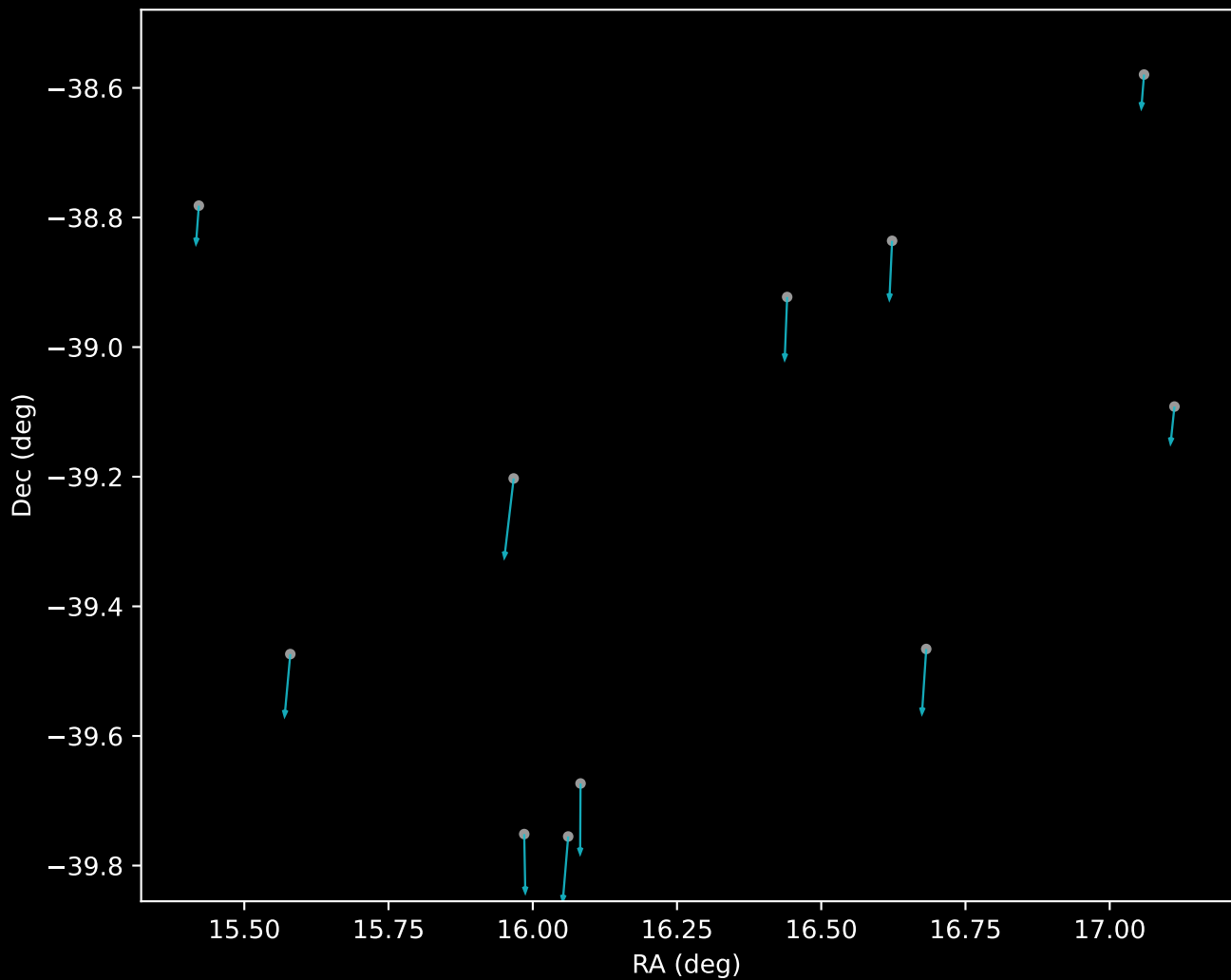
APOGEE DR17 Cluster 18 Proper Motion Vectors (n=11)
